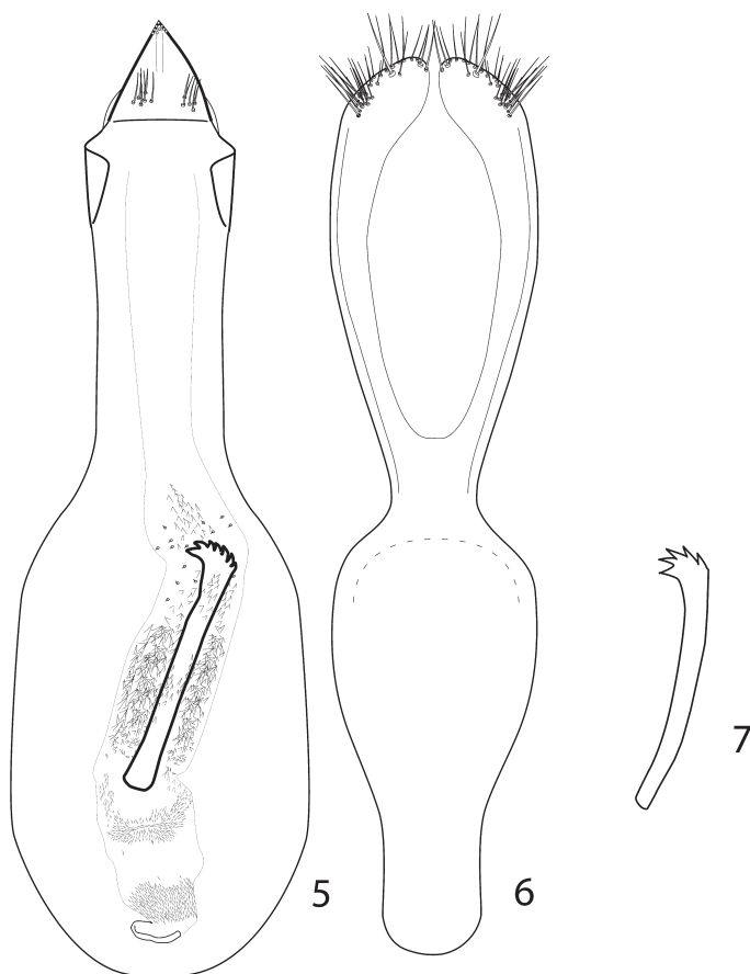
5-6. male genitalia of Bruchidius inconstitus , ventral view: 5 – median lobe; 6 – lateral lobe and tegminal strut; 7 – Bruchidius inexpectatus , sclerite of internal sac (after DECELLE, 1971)
